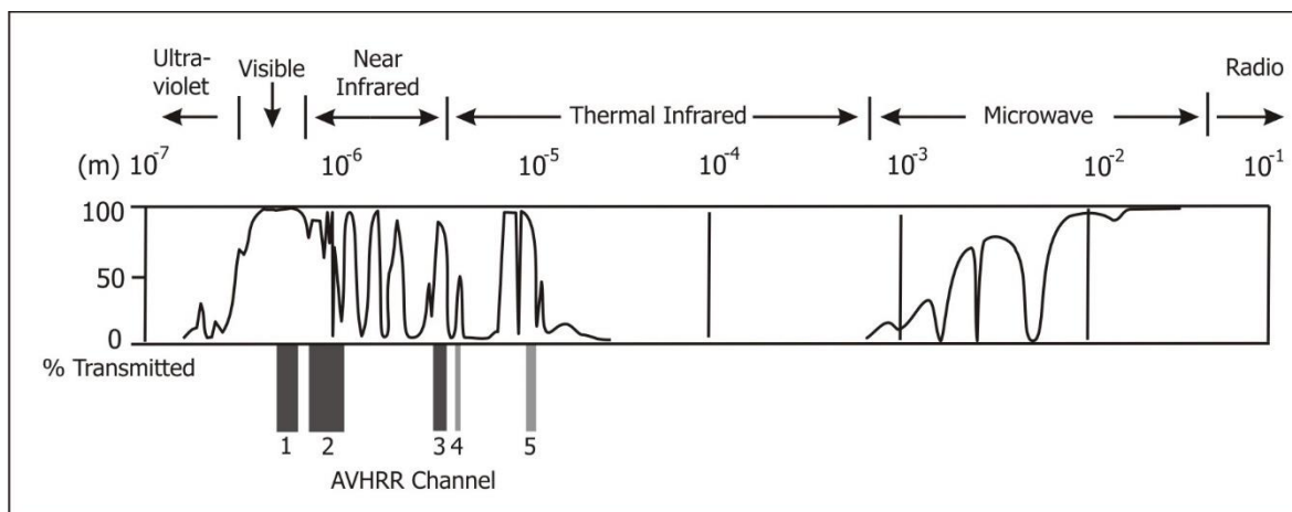
รูปที่ 11 Transmissivity of the Atmosphere and the Spectral Range of Five Main Sensors on the Advanced Very High Resolution Radiometer (AVHRR)
